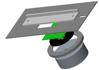
ALIGNMENT PLATE AND DEFINITION GASKET STACK-UP
